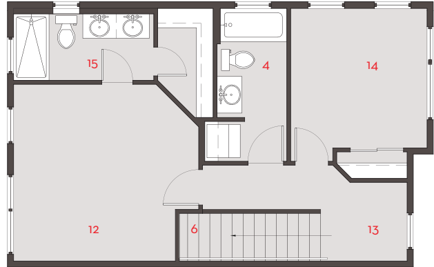
FLOOR PLAN LEVEL 3
