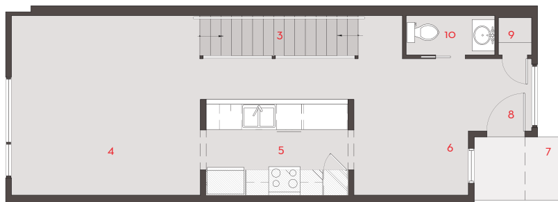
FLOOR PLAN LEVEL 3
