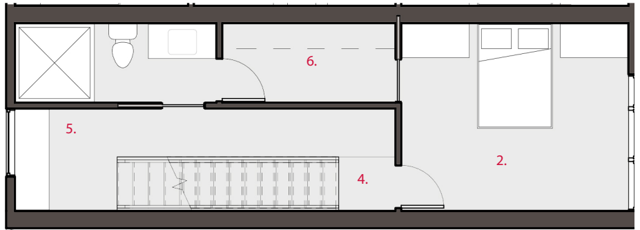
FLOOR 3
